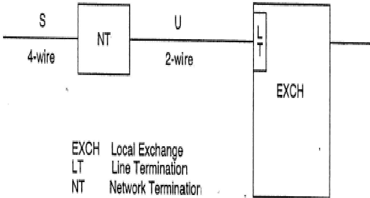
Fig. 2.9: Basic access netw termination
