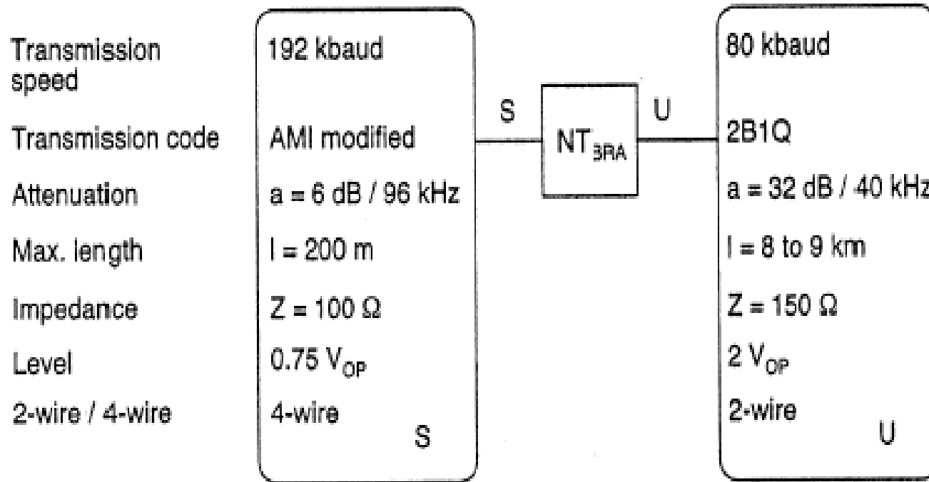
Fig. 2.11: Comparison between S and U interfaces
