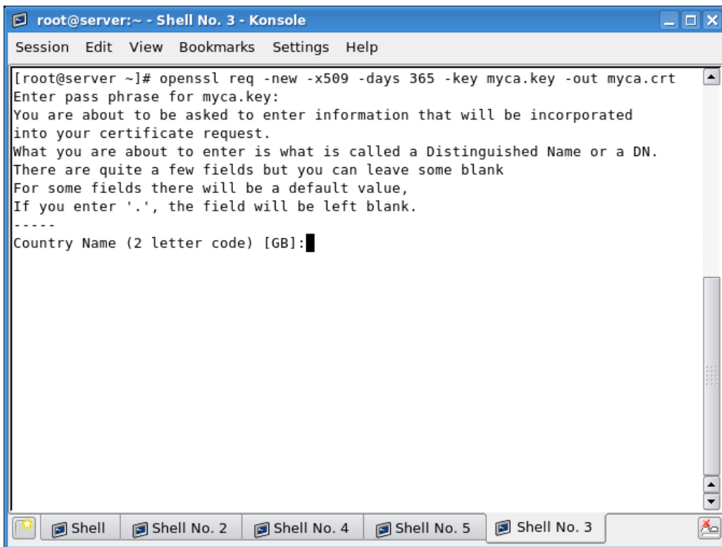
Figure 57: Creating new certificate
