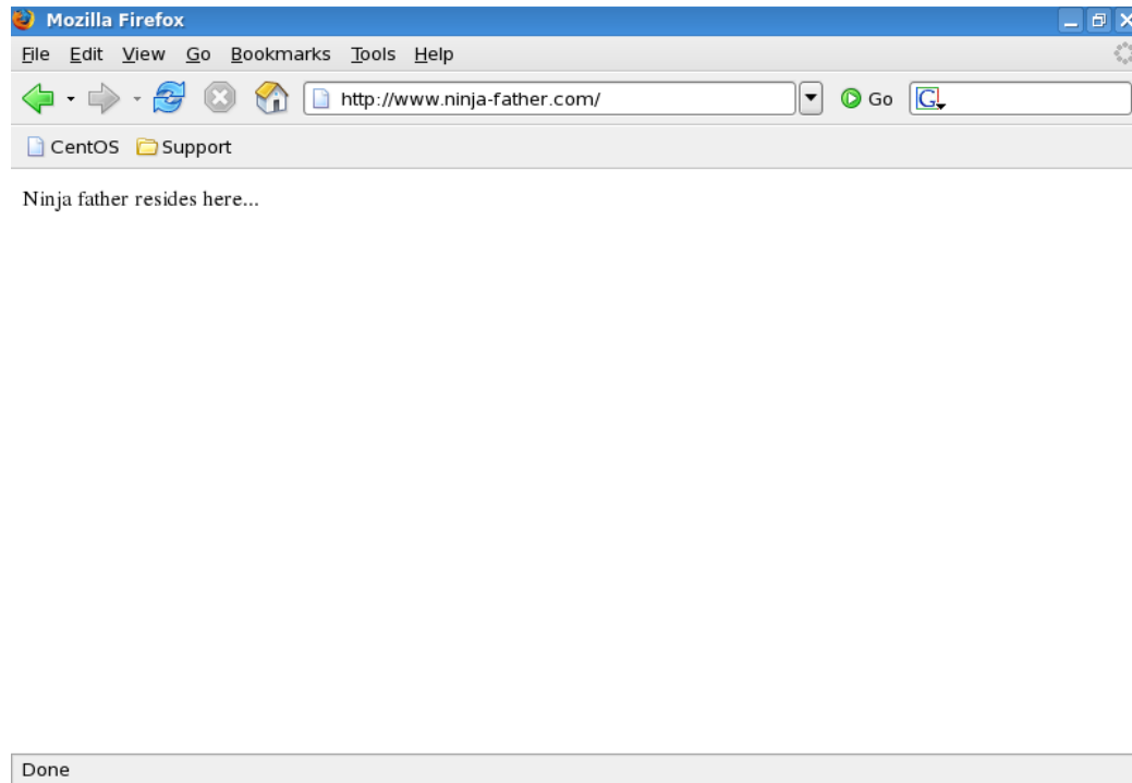
Figure 34: www.ninja-father.com
