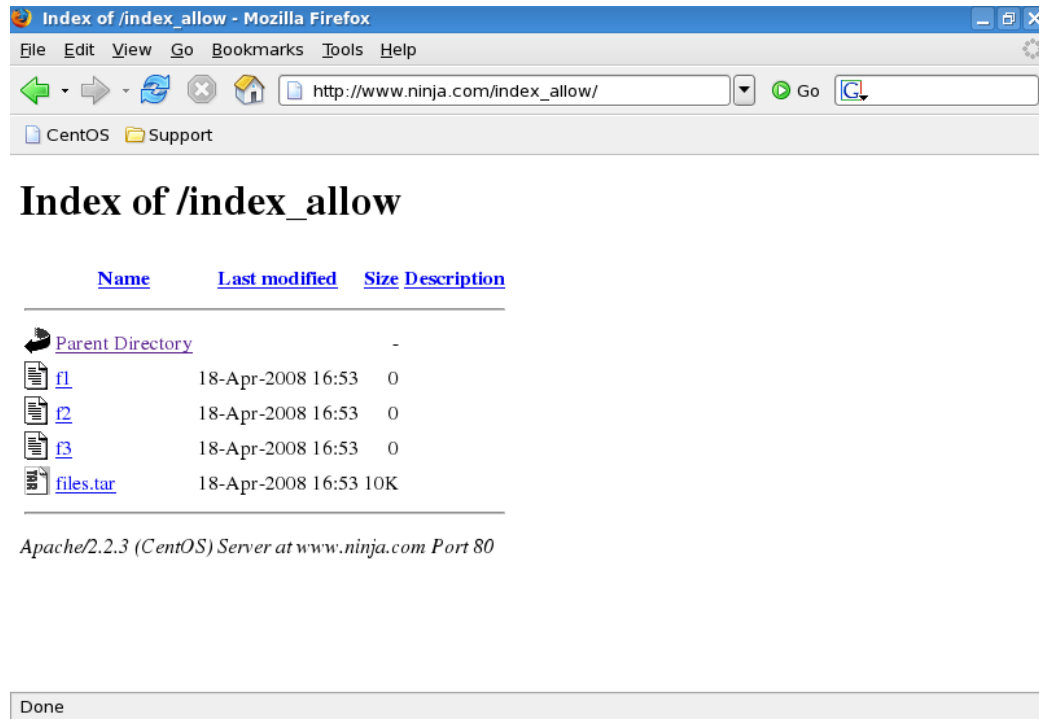
Figure 24: index_allow example
