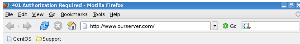
Figure 49: Authorization required
