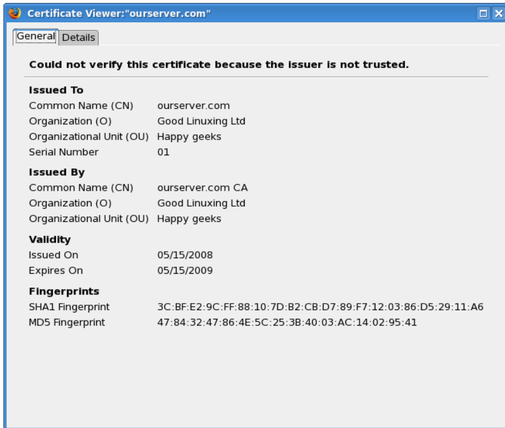
Figure 71: Certificate Viewer
