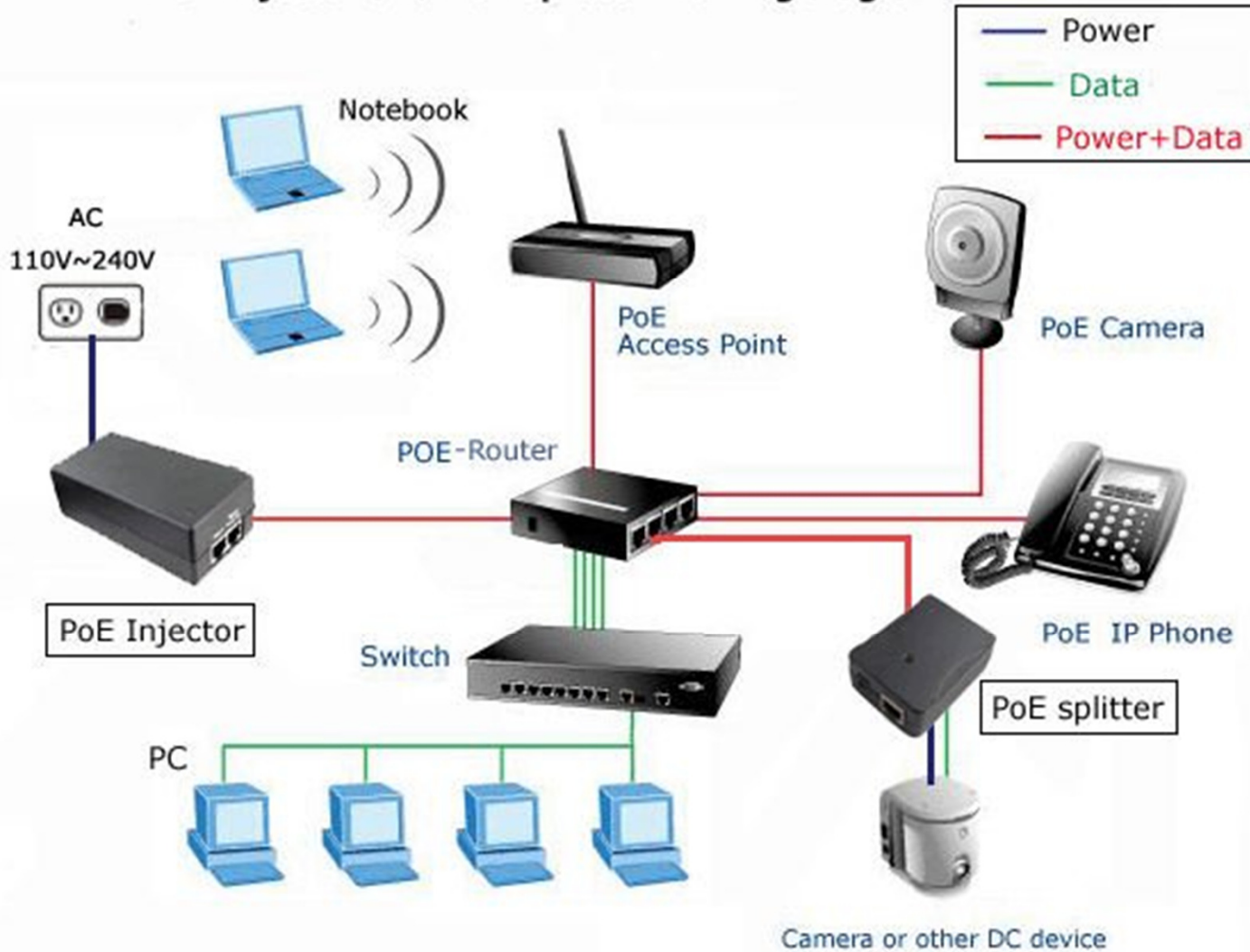
PoE Injector and PoE Splitter working diagram
